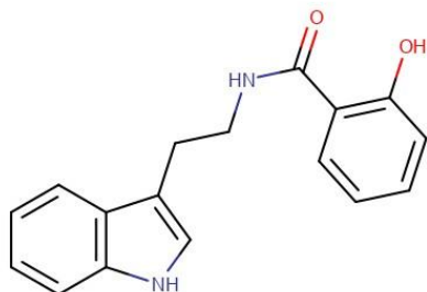
N-salicyloyl tryptamine
