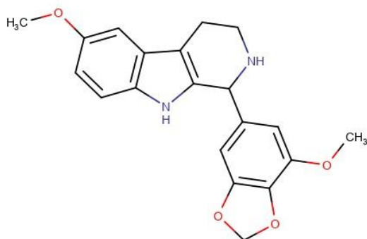
6-MeO-1-(3-methoxy-4,5-methylenedioxyphenyl)THBC
