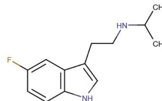
Name: [2-(5-fluoro-1H-indol-3-yl)ethyl](propan-2-yl)amine Molecular weight: 220.29 Formula: C 13 H 17 FN 2
