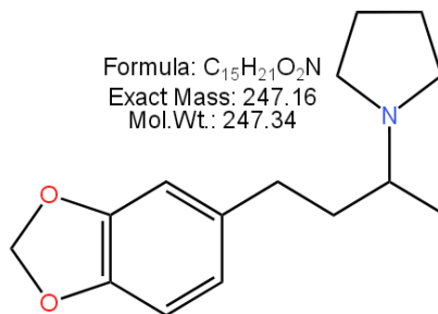
1-[4-(2H-1,3-benzodioxol-5-yl)]butan-2-yl]pyrrolidine
